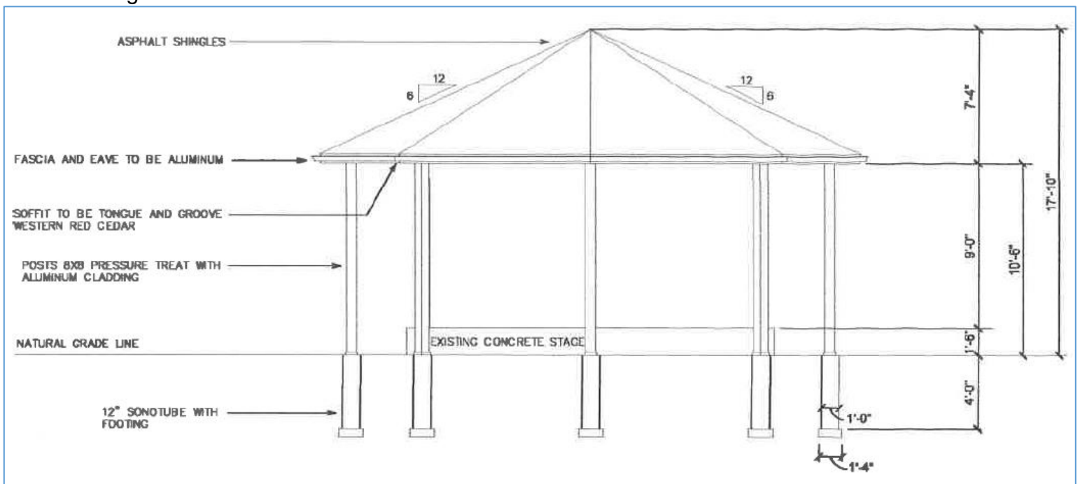
Figure 2: Side View of Structure with Dimensions
