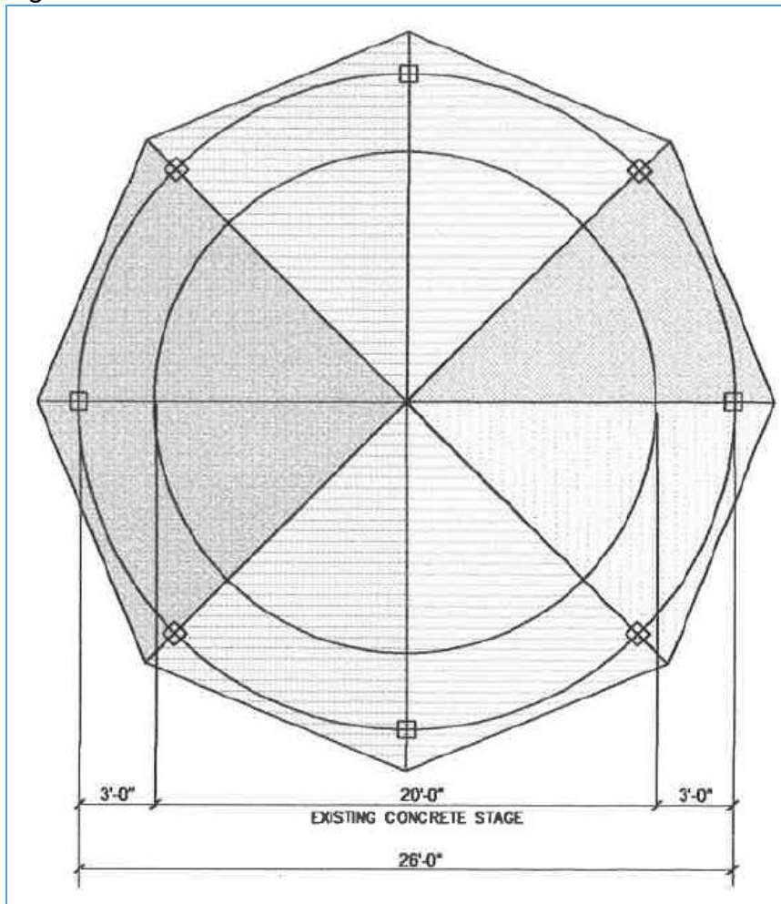
Figure 3: Aerial View of Band Cover with Dimensions
