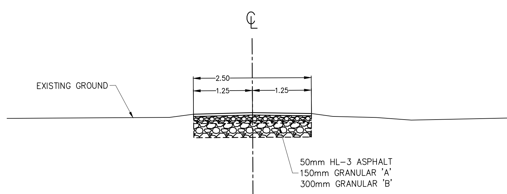
(A) ASPHALT SIDEWALK CROSS-SECTION DETAIL SCALE: 1:30
